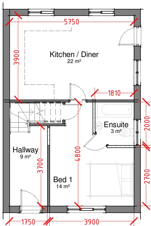
Proposed Ground 1 : 100
