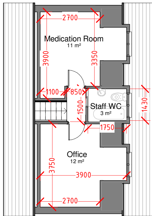
Proposed First 1 : 100
