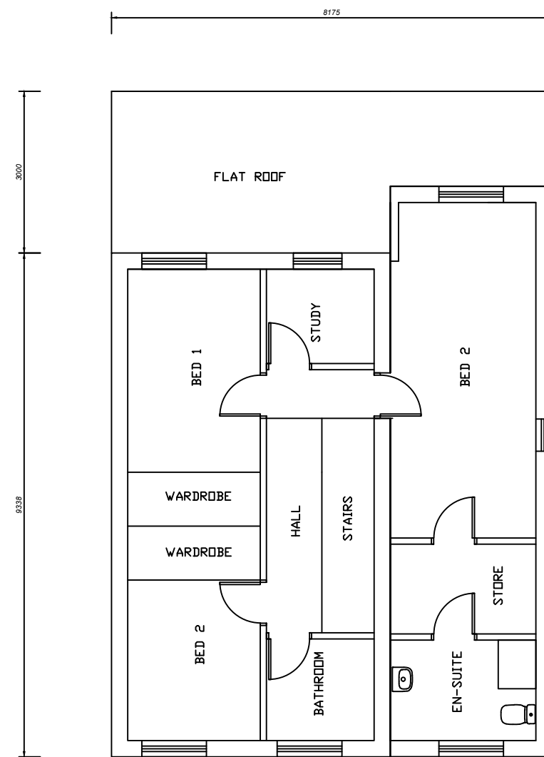
PROPOSED FF
