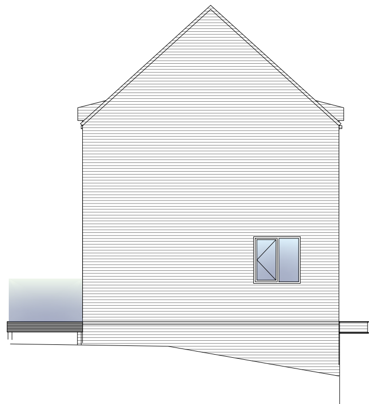
South elevation
