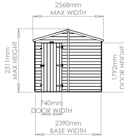
SOUTH ELEVATION
