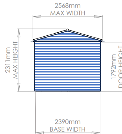
NORTH ELEVATION
