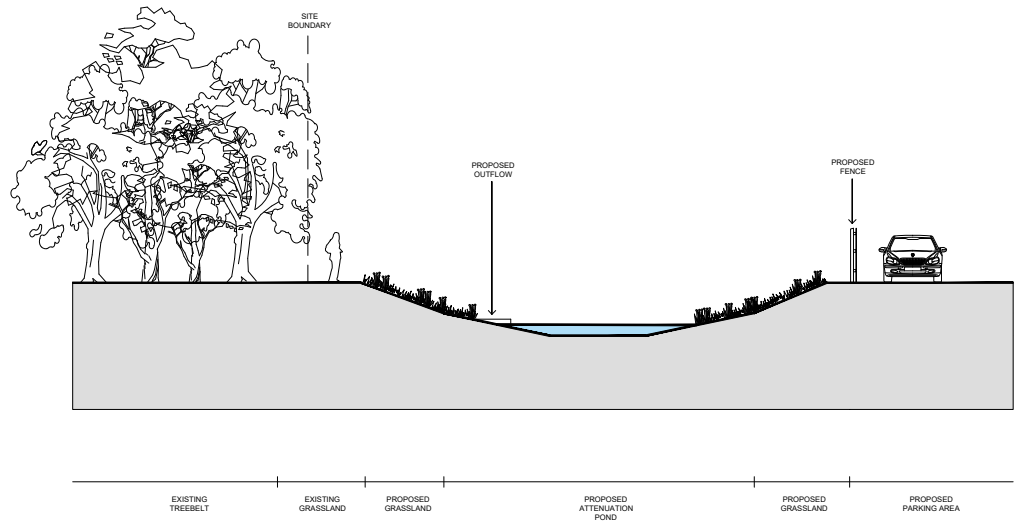
SECTION B
