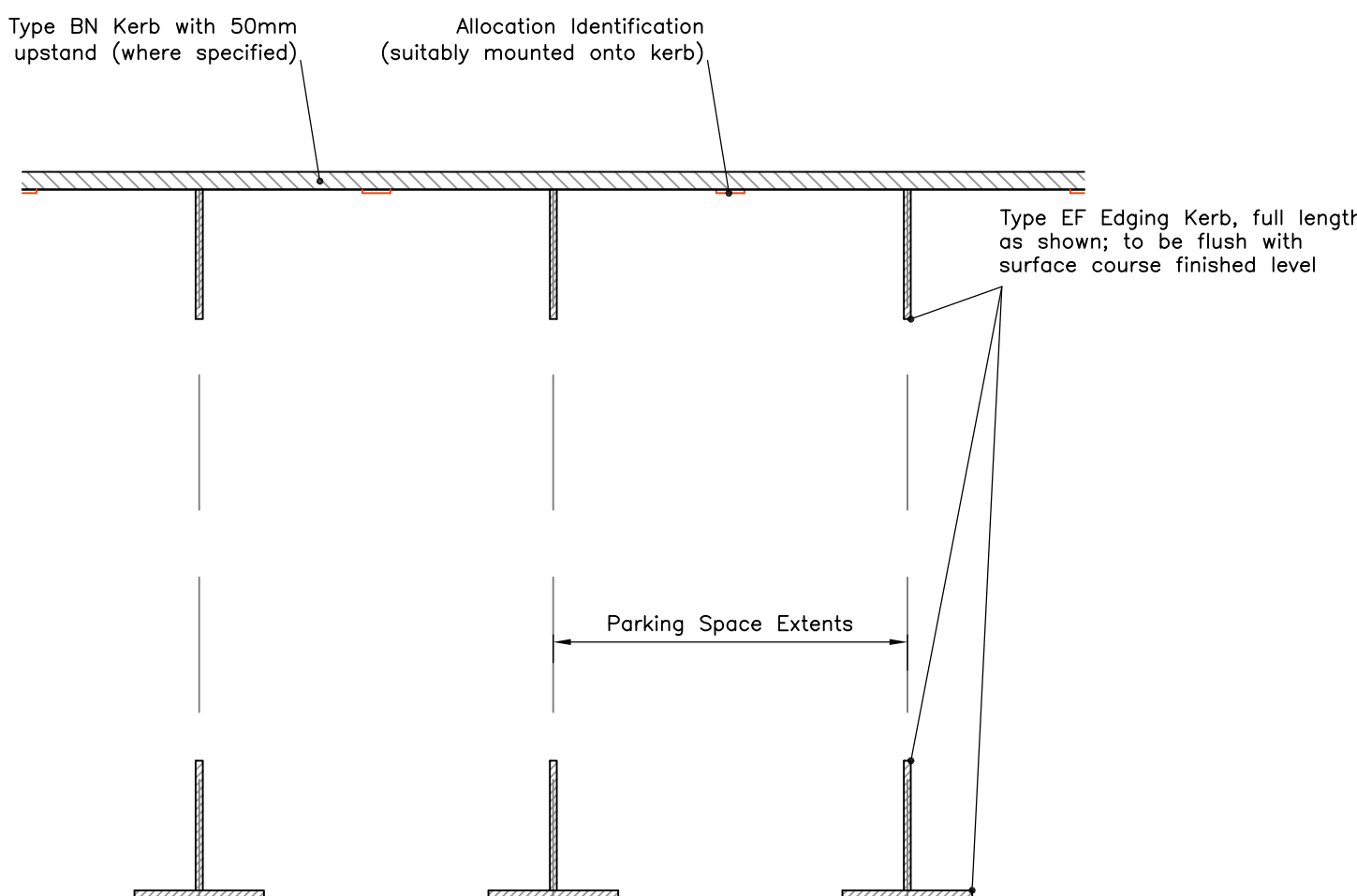
Parking Courtyard Delineation Scale 1:50
