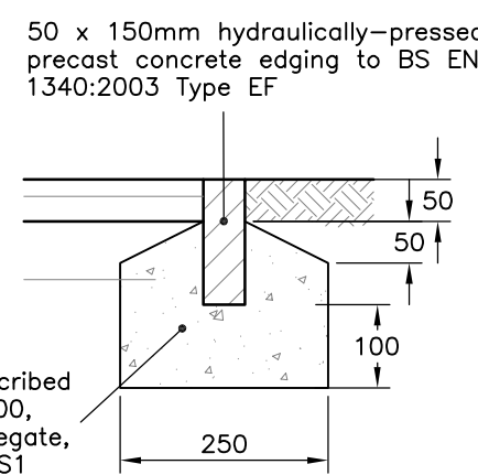
Type EF Edging (as HCC Drawing No. HCC11/C/045) Scale 1:10
