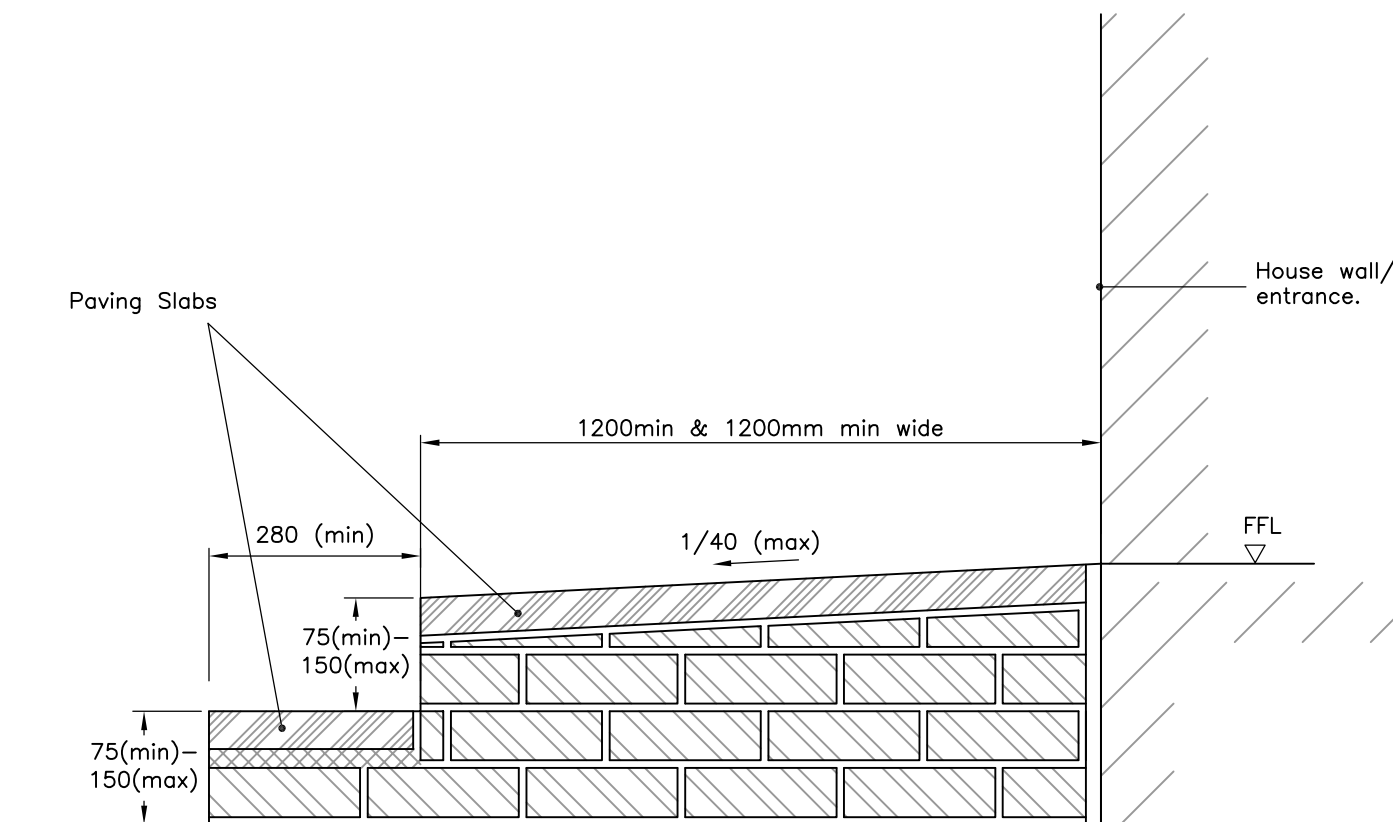
Part M Stepped Approach to Level Access Detail n.t.s
