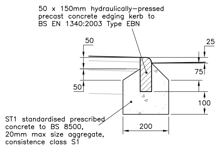
Type EBN Edging Kerb Scale 1:10
