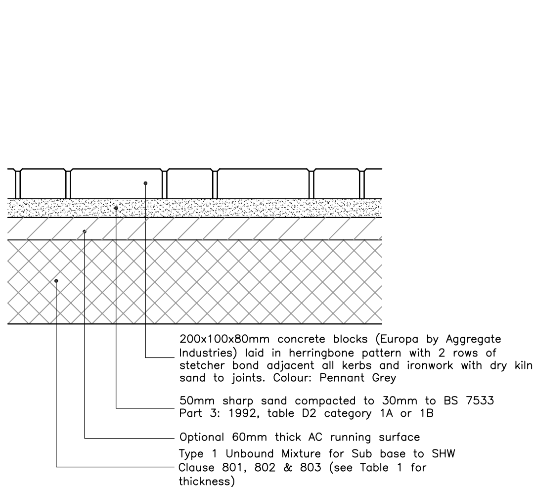
Block Paved Driveway Scale 1:10
