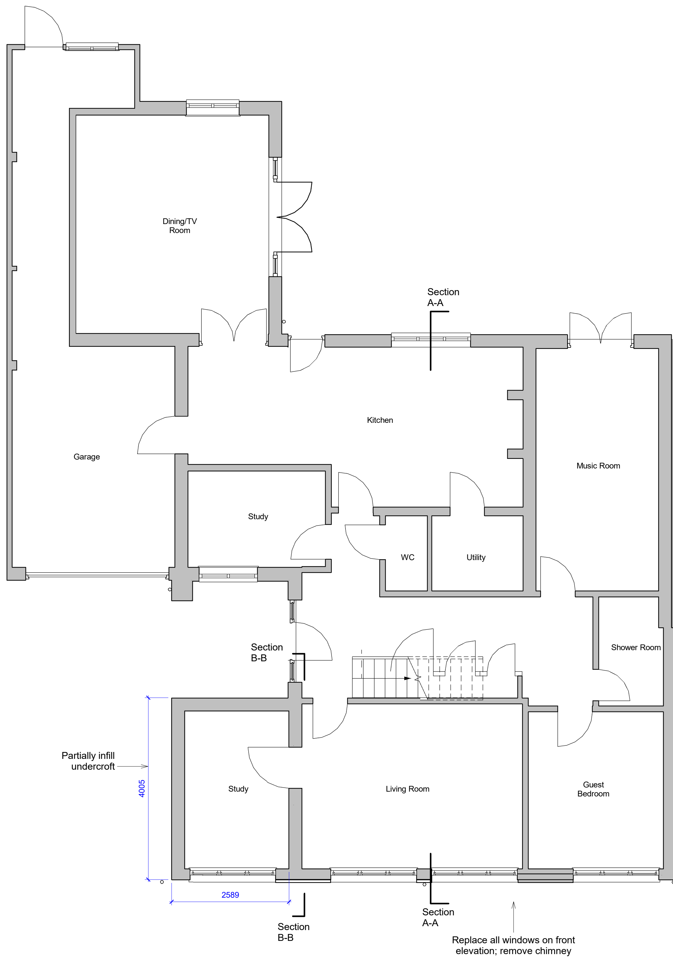
Ground Floor Plan as Proposed 1:50
