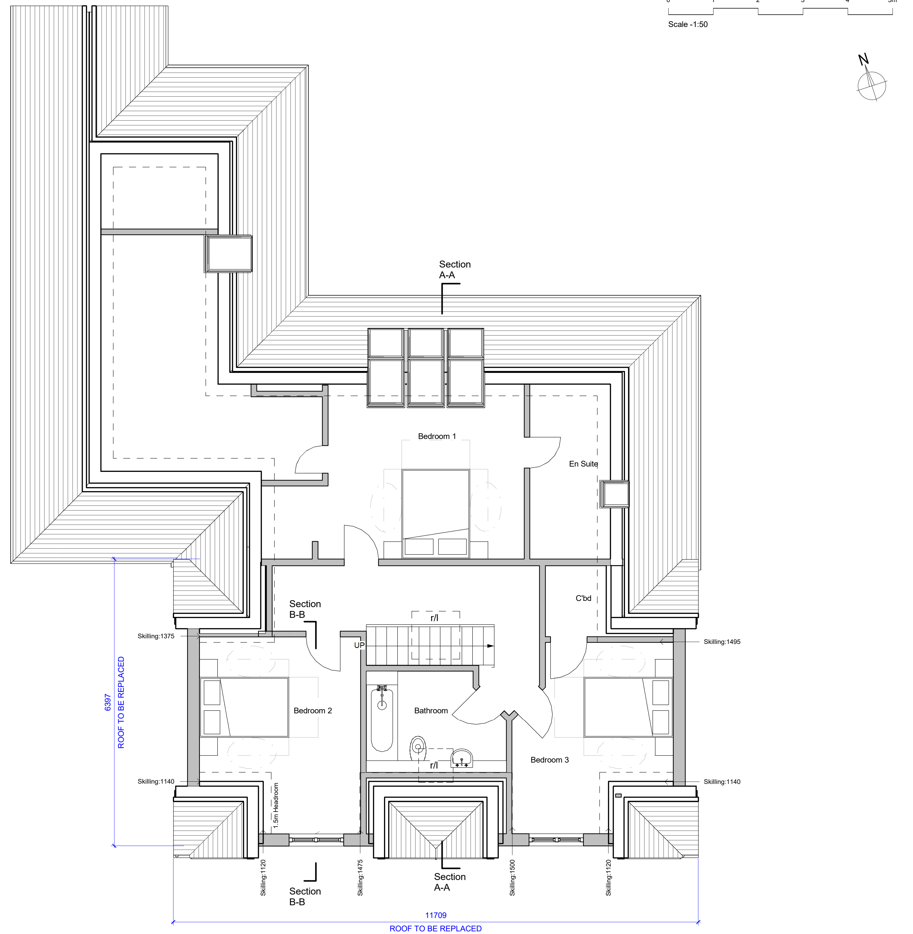
First Floor Plan as Proposed 1:50
