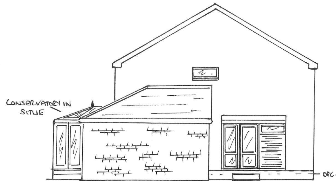
EXISTING SIDE ELEVATION (AS VIEWED FROM BROWNSHOLME CLOSE) SCALE 1:100
