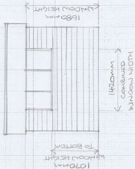
SOUTH ELEVATION
