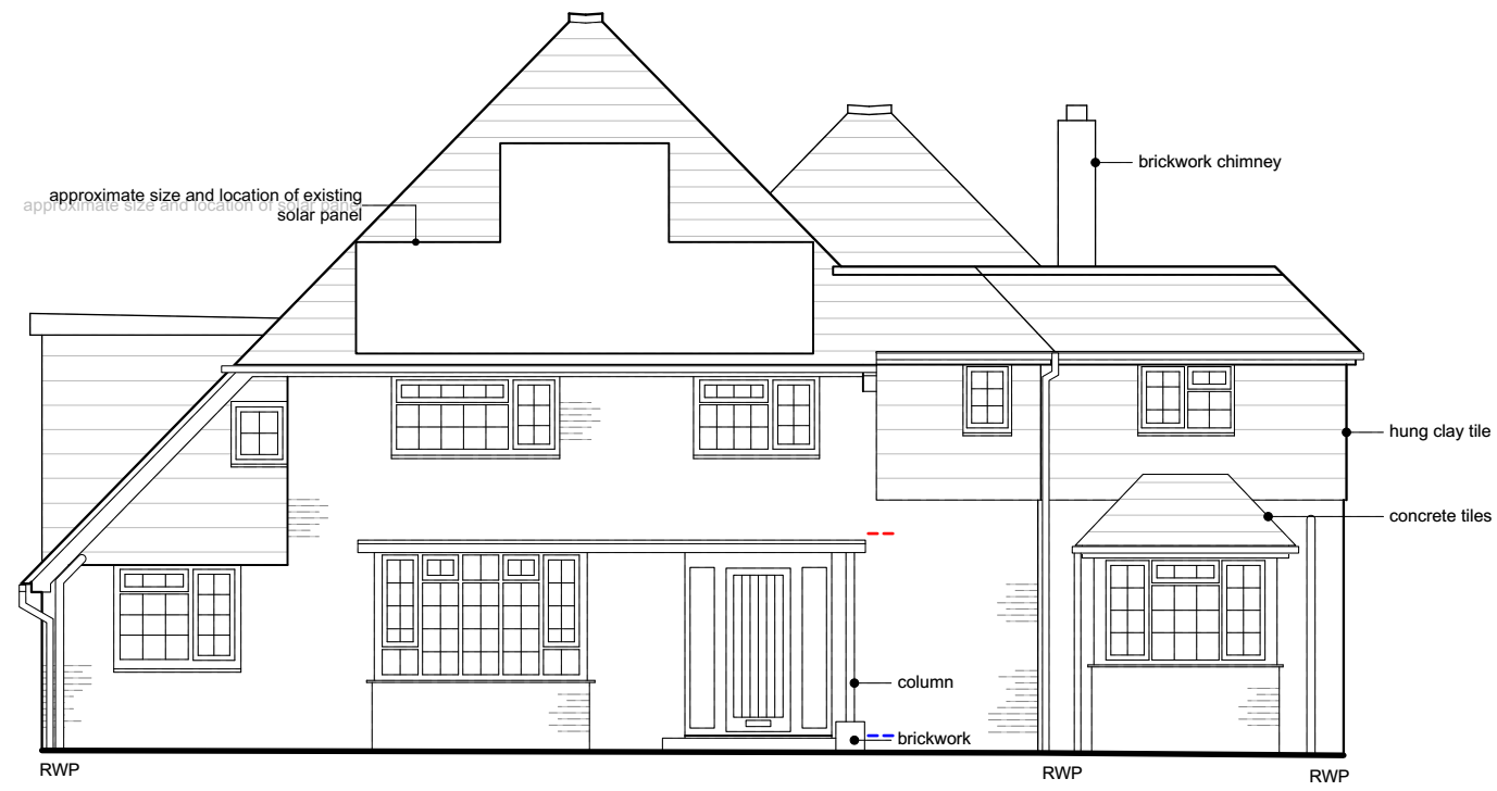
FRONT ELEVATION
