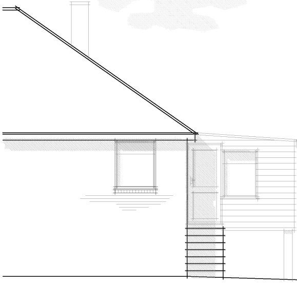
EXISTING PART SIDE ELEVATION (facing due north) SCALE 1:100
