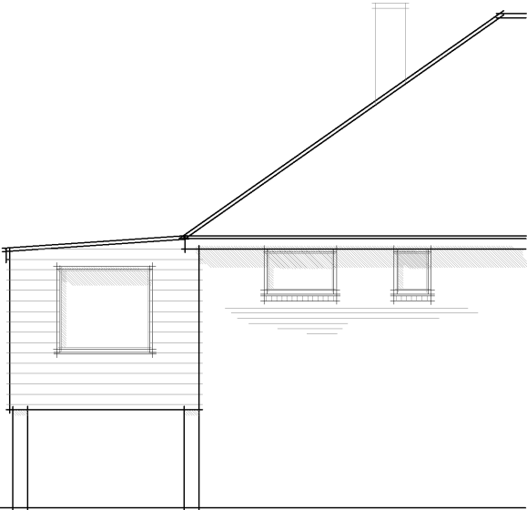
EXISTING PART SIDE ELEVATION (facing due south) SCALE 1:100
