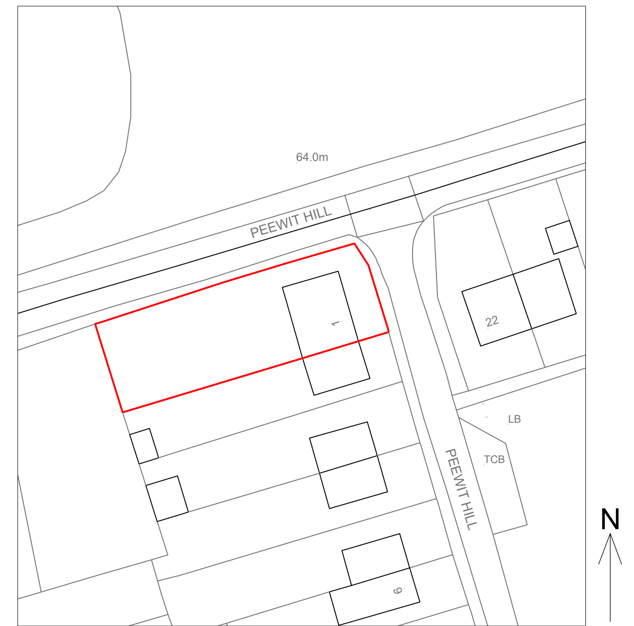
Block Plan - As Proposed 1:500
