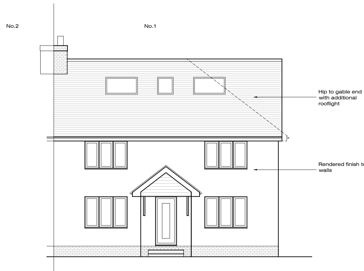
North-East (Front) Elevation - As Proposed
