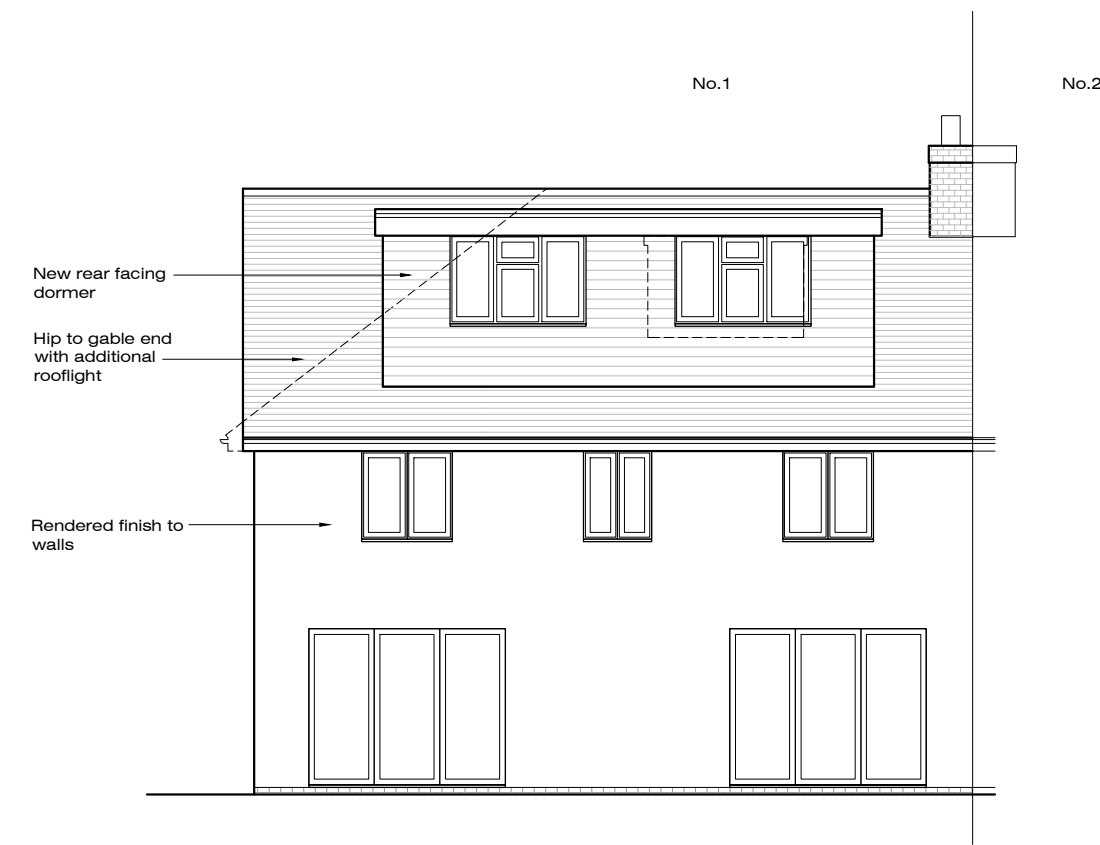
South-West (Rear) Elevation - As Proposed
