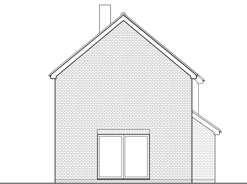
East (Side) Elevation - As Existing
