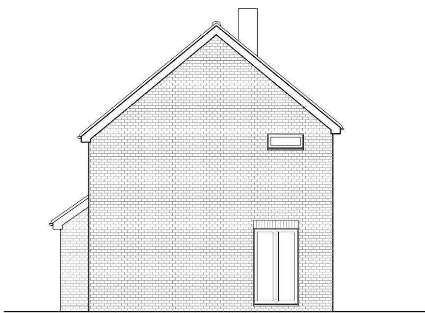
West (Side) Elevation - As Existing
