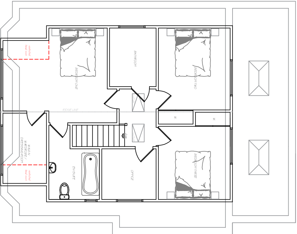
Proposed First Floor Plan | : 100 @ A3
