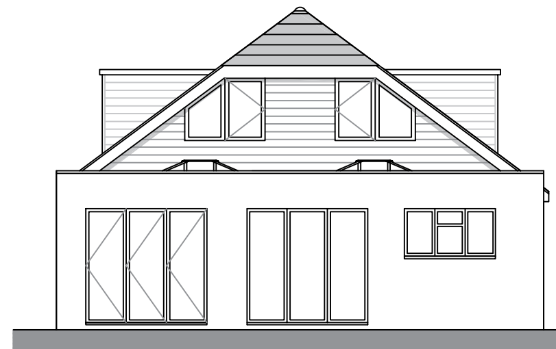
Proposed Rear Elevation 1:100 @ A3
