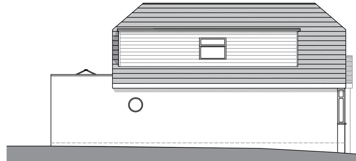
Proposed Side Elevation 1:100 @ A3
