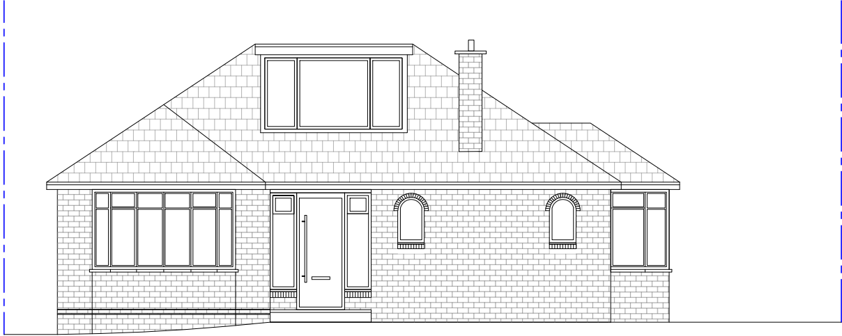
Existing Front Elevation 1:100 @A3
