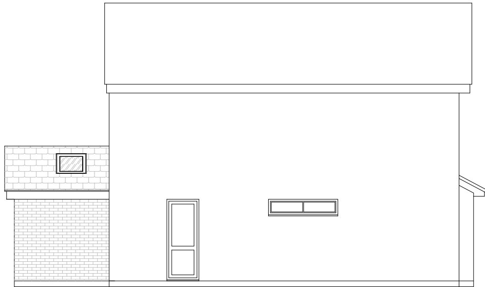
West Elevation
