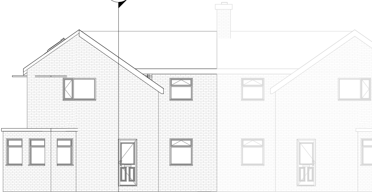
Proposed Elevation-Front
