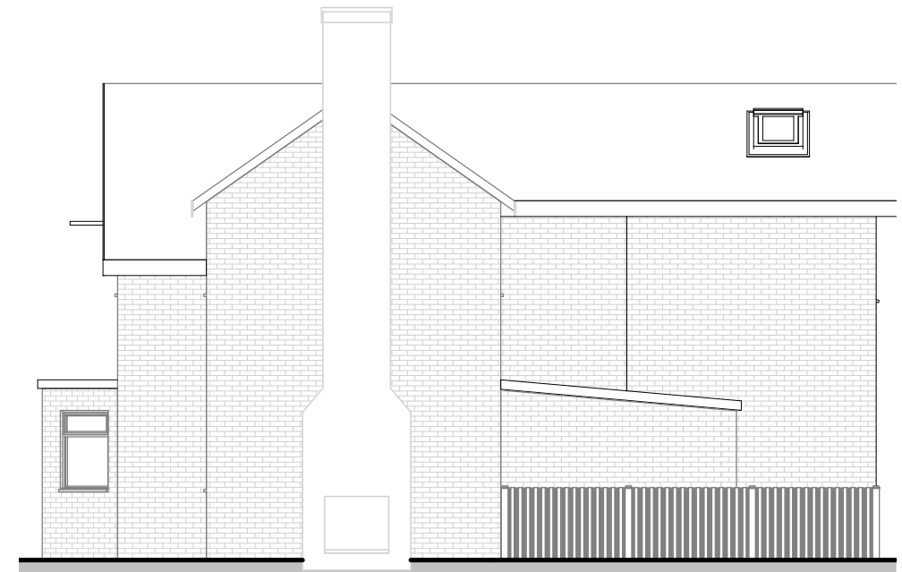
Proposed Elevation-Right side
