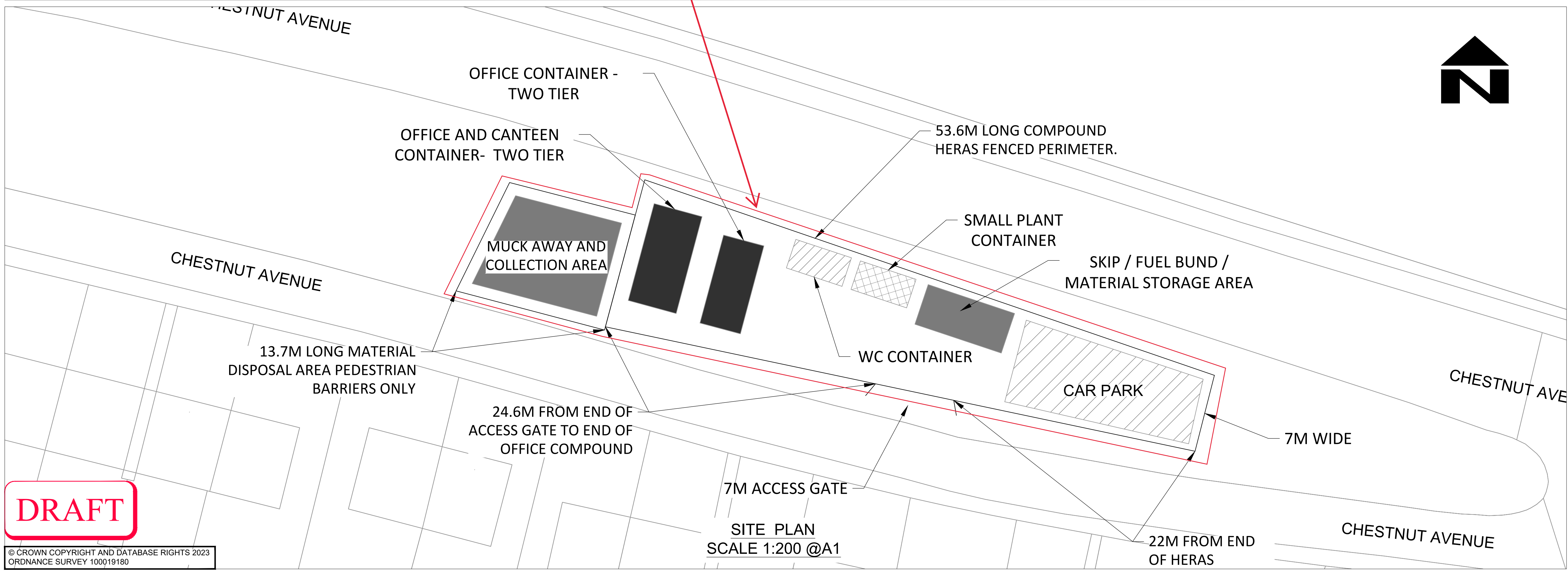
SITE LOCATION PLAN SCALE 1:1250 @A1
