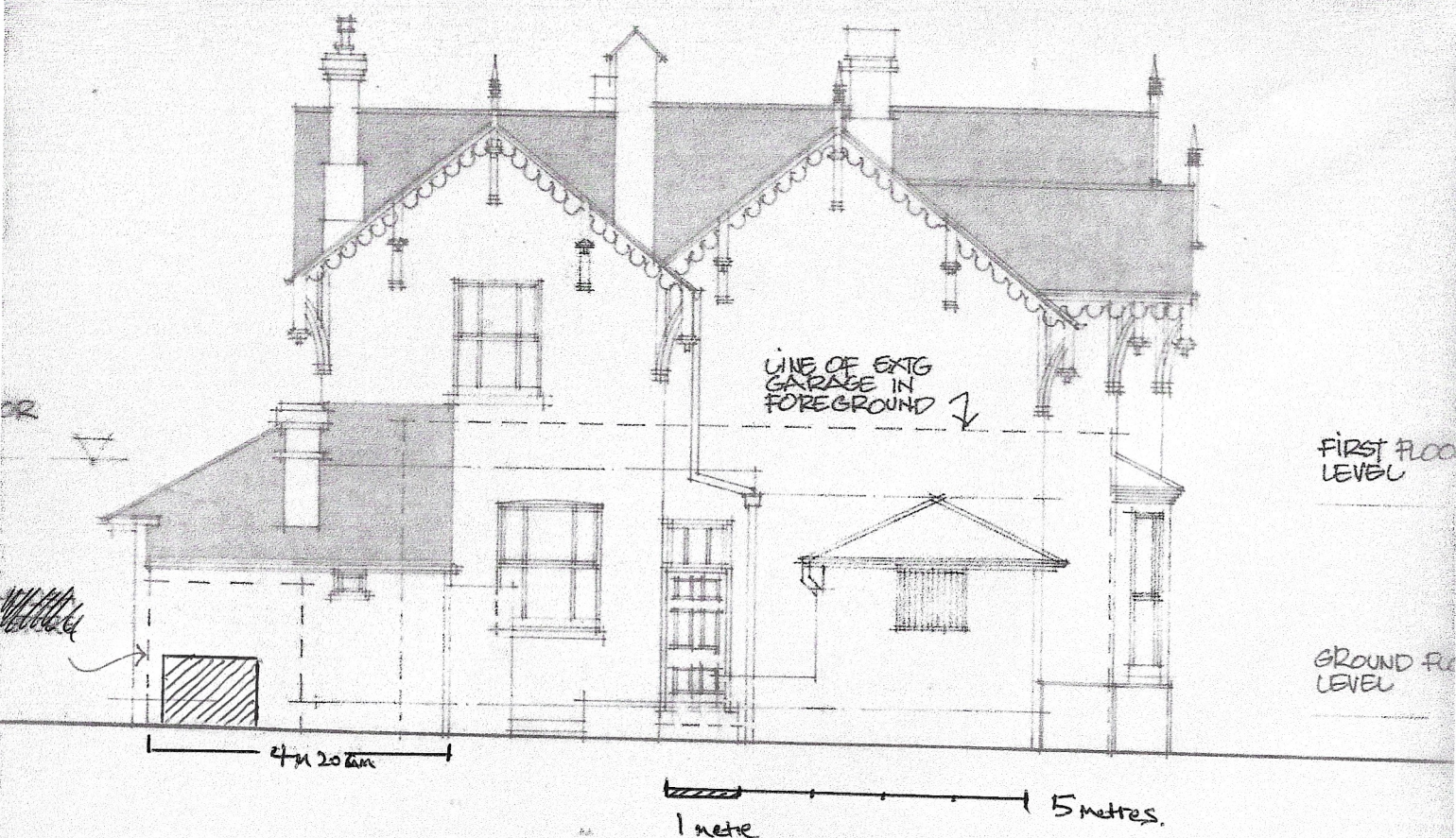
Side elevation - EAST
