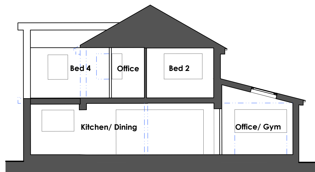
SECTION B-B
