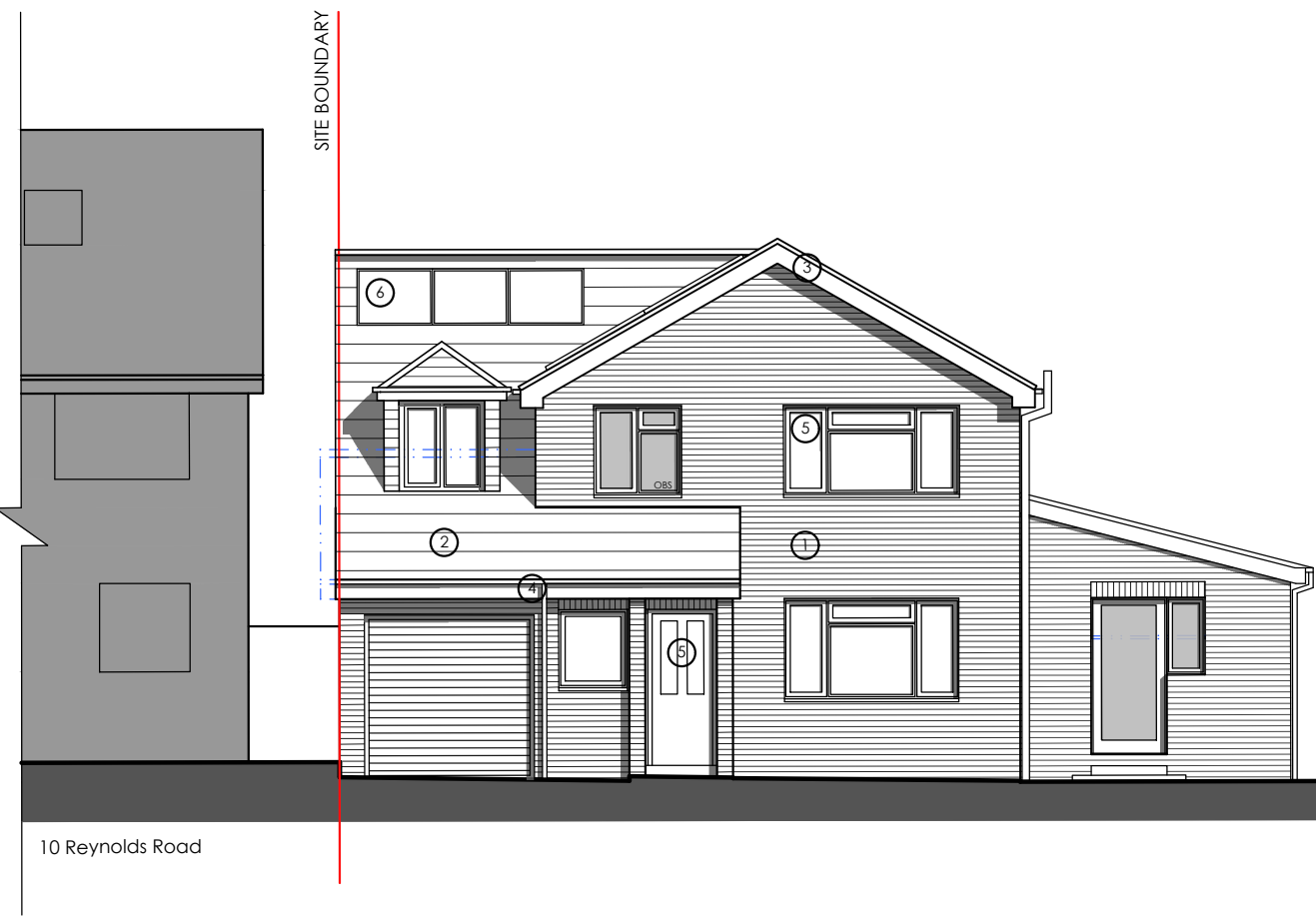
SOUTH ELEVATION
