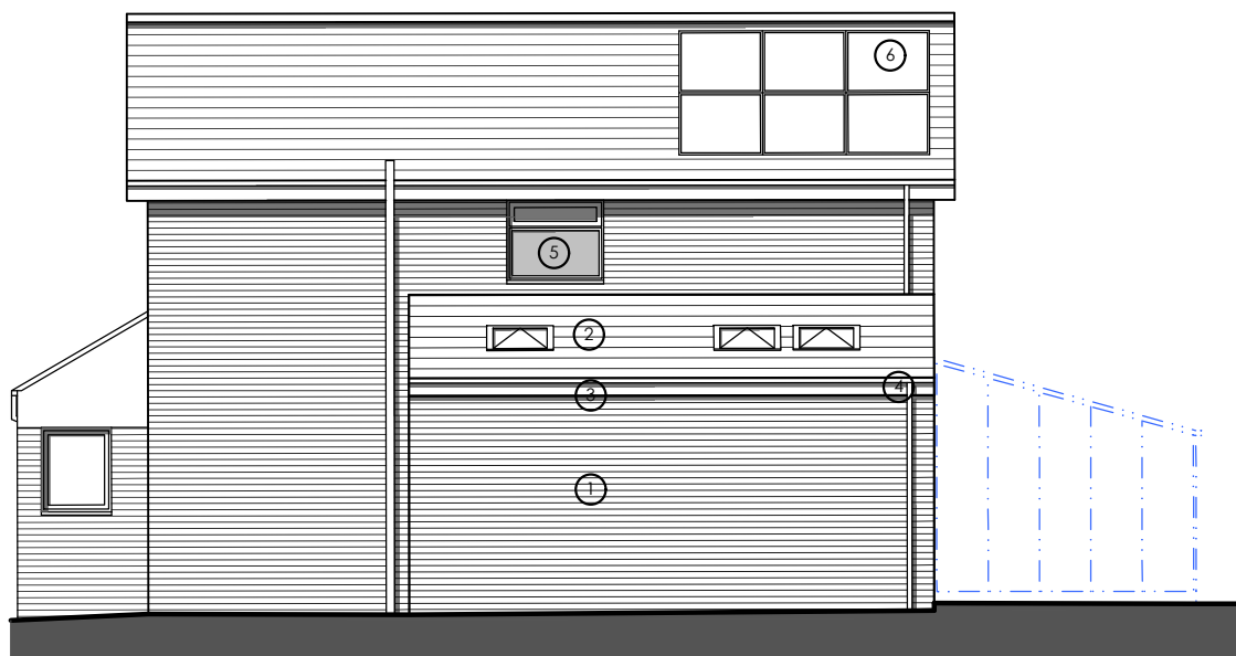
EAST ELEVATION
