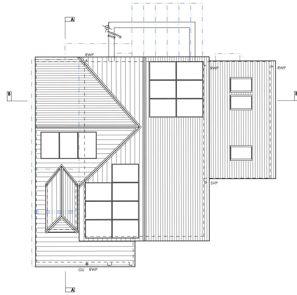
ROOF PLAN
