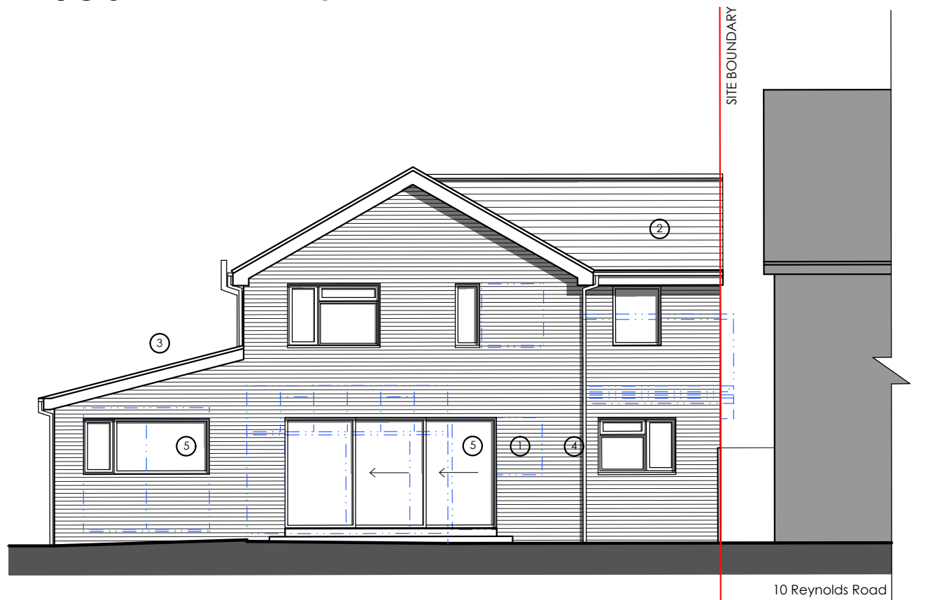
SOUTH ELEVATION
