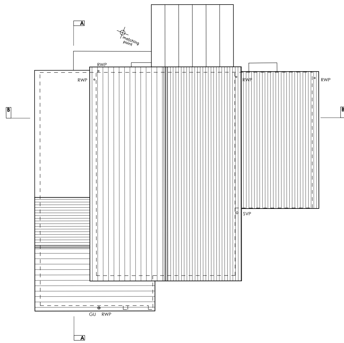
ROOF PLAN
