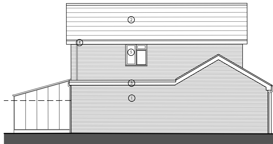
WEST ELEVATION
