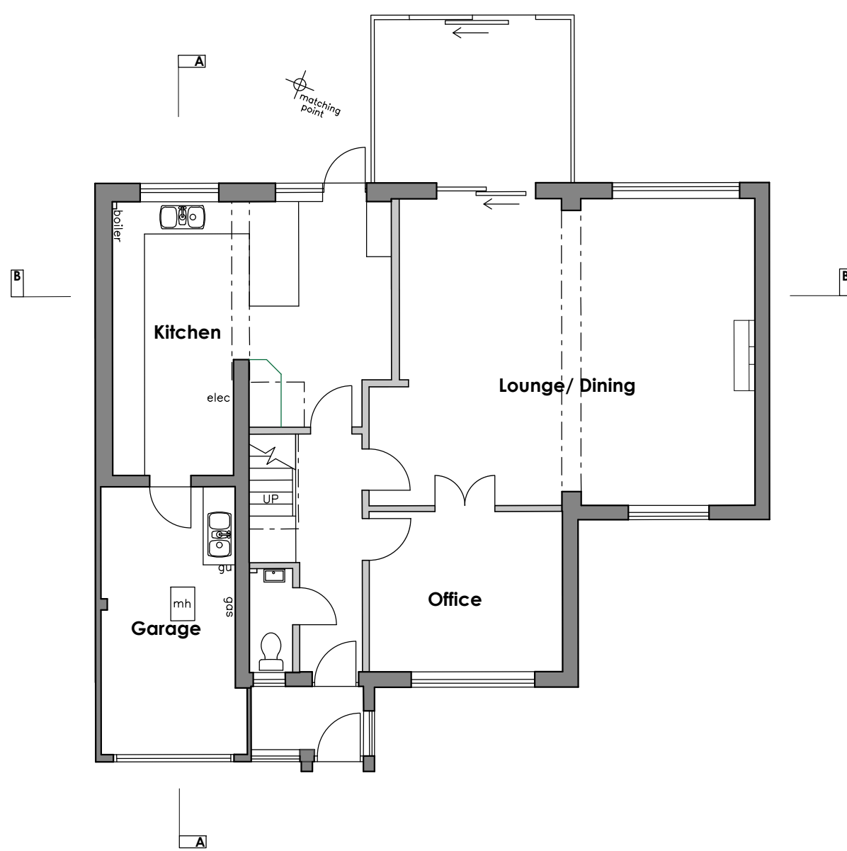
GROUND FLOOR
