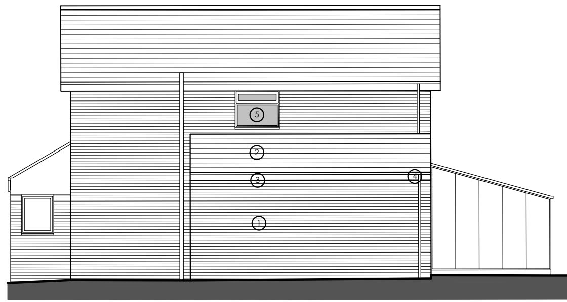
EAST ELEVATION
