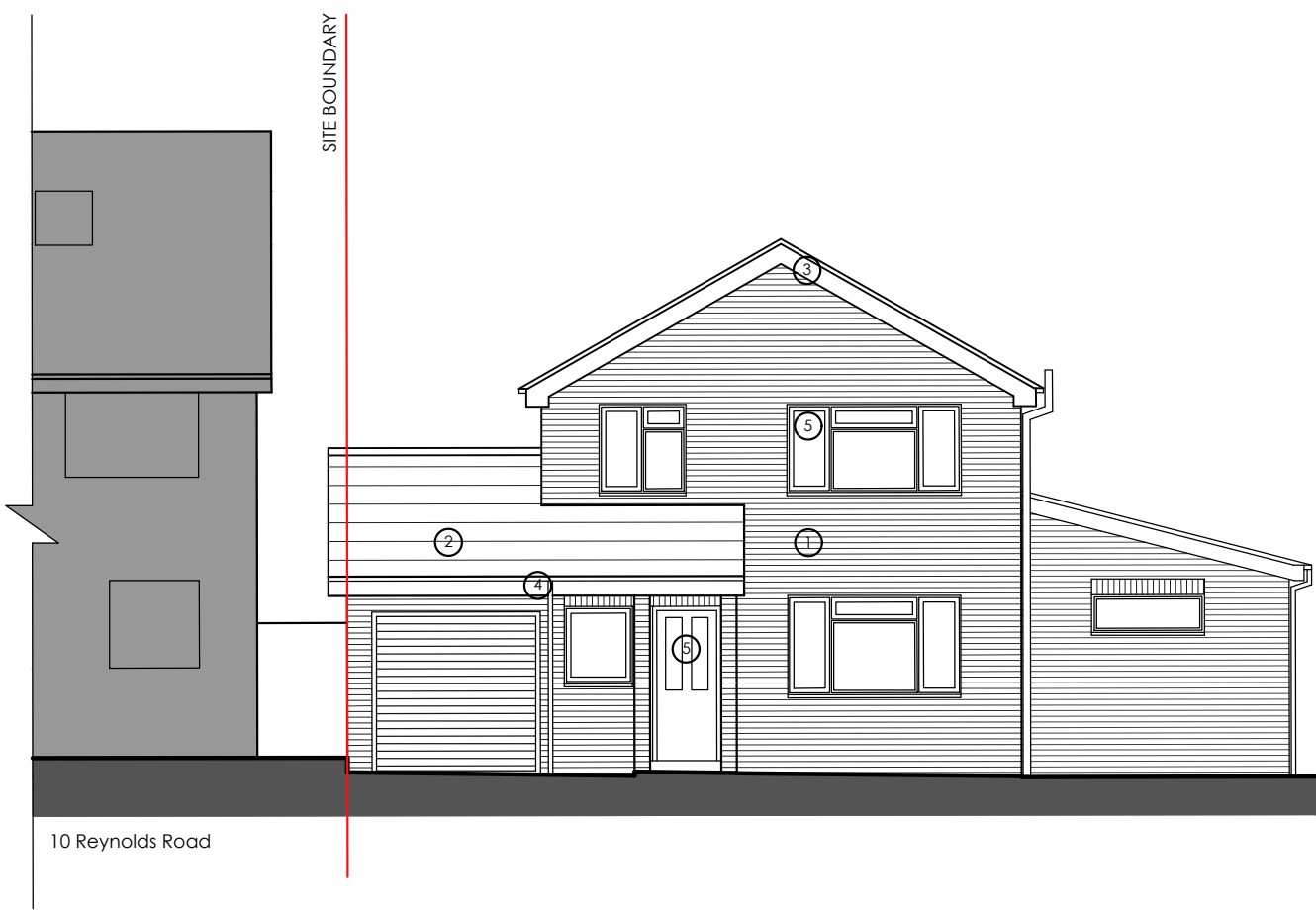
SOUTH ELEVATION
