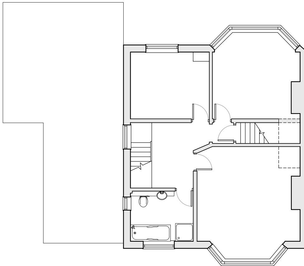
Existing First Floor - 1:100
