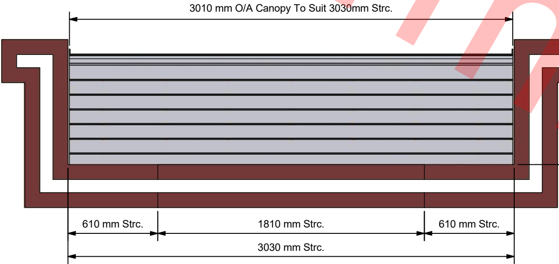
Reflected Plan Elevation (View From Beneath) ( 1 : 25 )
