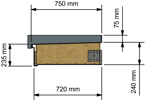
Auxiliary View ( 1 : 35 )
