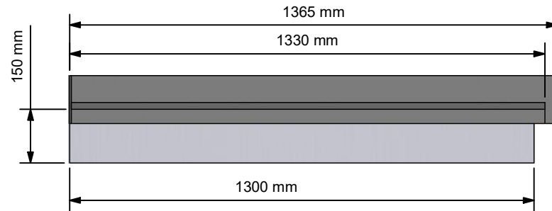
Front Elevation ( 1 : 15 )
