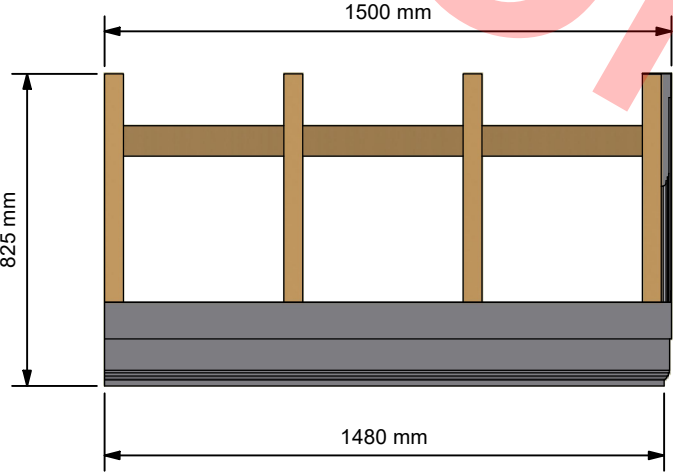
Front Elevation ( 1 : 20 )
