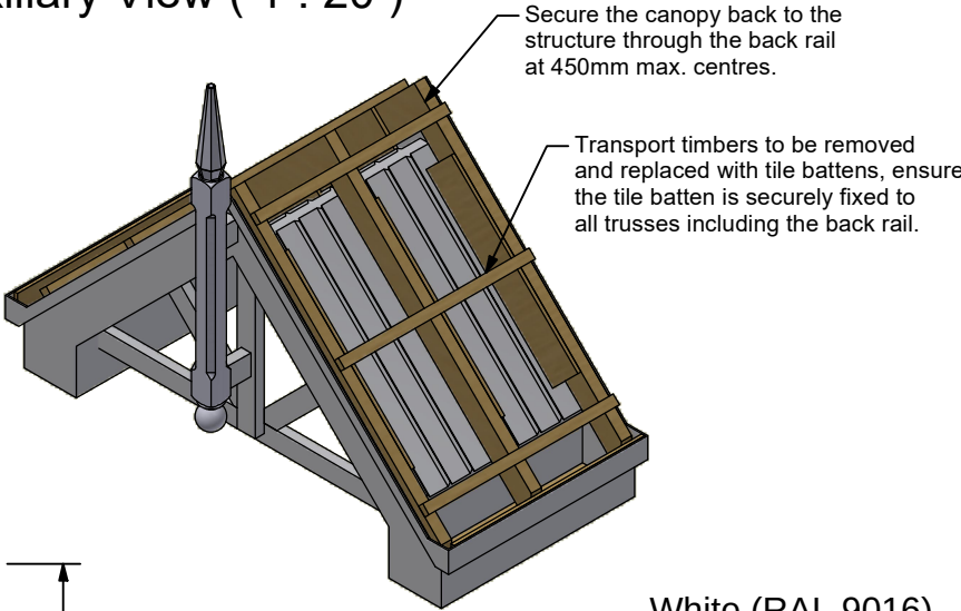
Auxiliary View ( 1 : 20 )
