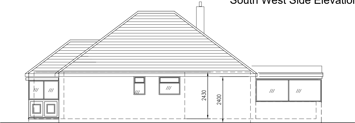
South West Side Elevation
