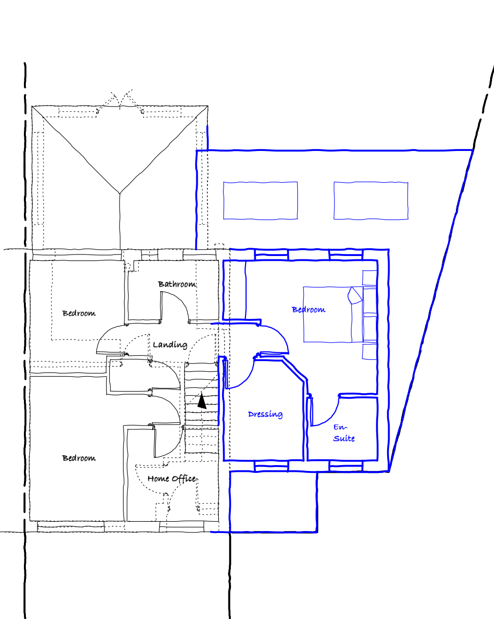
Proposed First Floor Plan 1:100 © MDT Design
