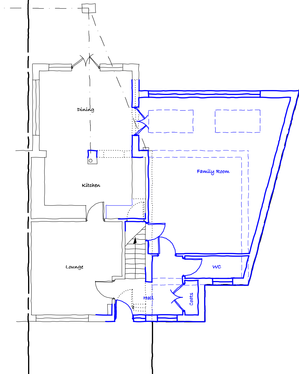
Proposed Ground Floor Plan 1:100 © MDT Design
