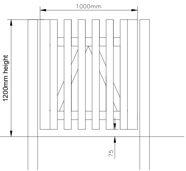
ELEVATION VIEWED FROM OUTSIDE
