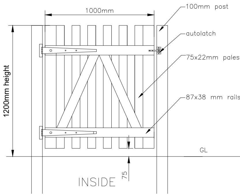
ELEVATION URBAN 1.2M BLACK PICKET FENCE WITH FLAT TOP PALES GATE VIEWED FROM INSIDE
