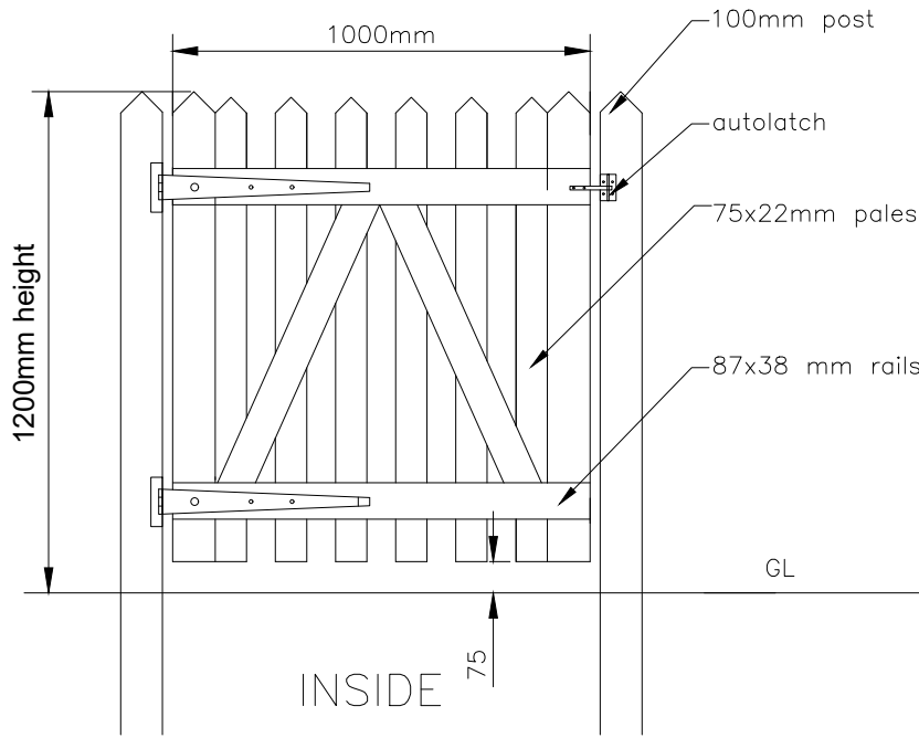
ELEVATION SUBURBAN 1.2M WHITE PICKET FENCE WITH POINTED PALES GATE VIEWED FROM INSIDE
