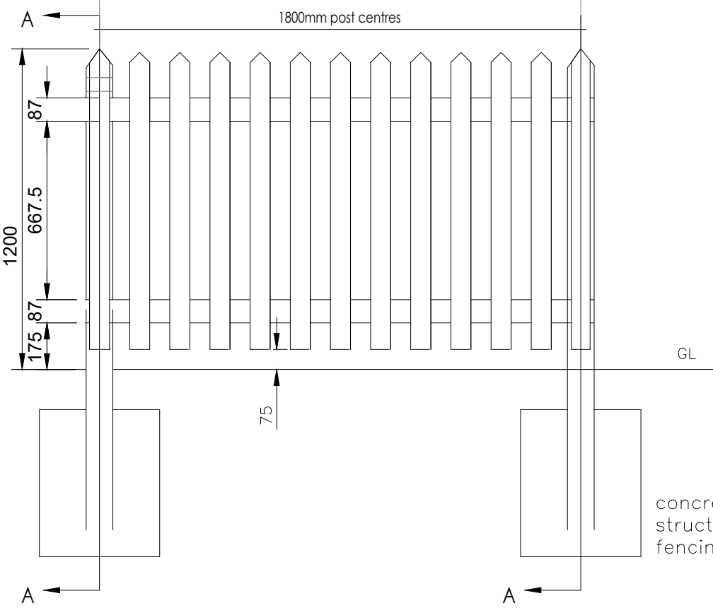
ELEVATION SUBURBAN 1.2M WHITE PICKET FENCE WITH POINTED PALES
