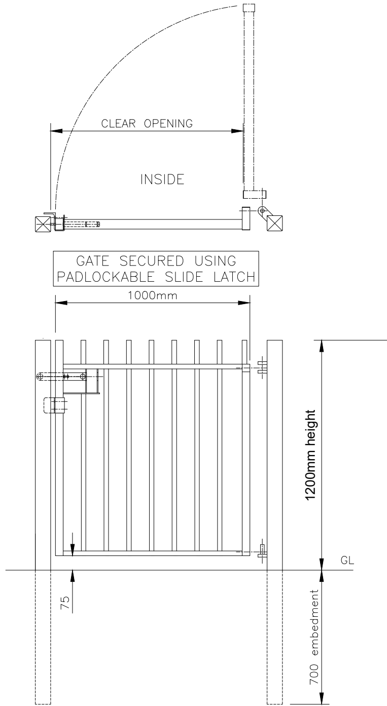
ELEVATION URBAN 1.2M STANDARD BLACK RAILINGS GATE VIEWED FROM OUTSIDE
