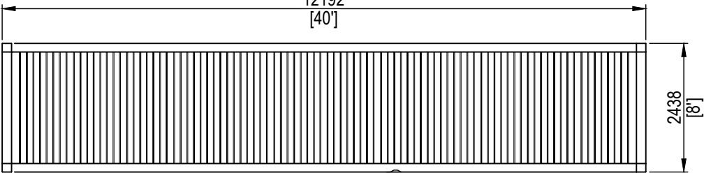
Typical Roof Plan
