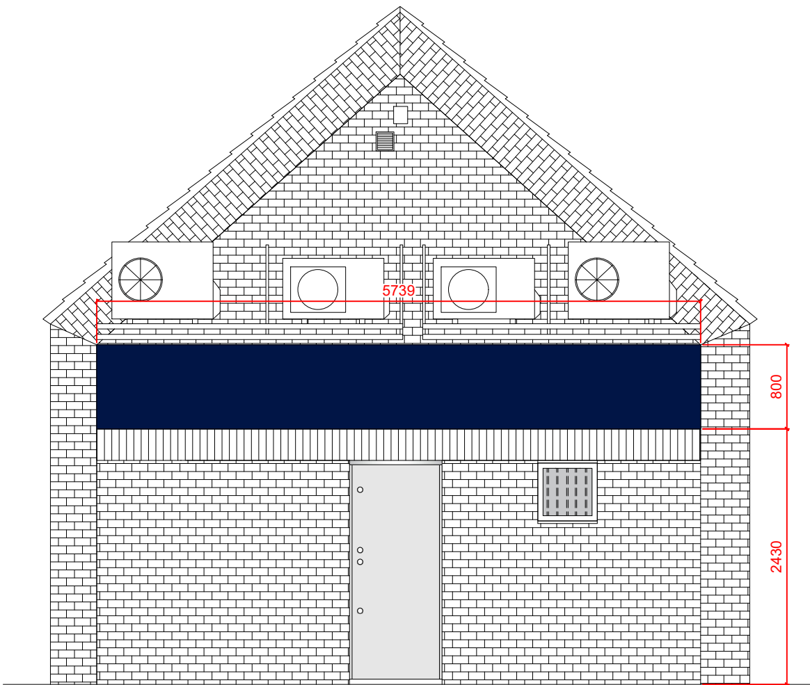
REAR ELEVATION
