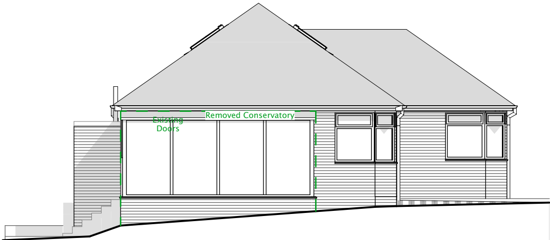
Side Elevation 1:100
