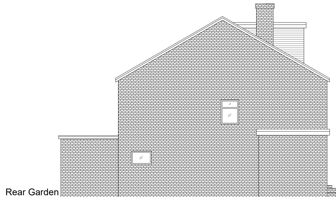
Existing West Elevation 1:100 @A3
