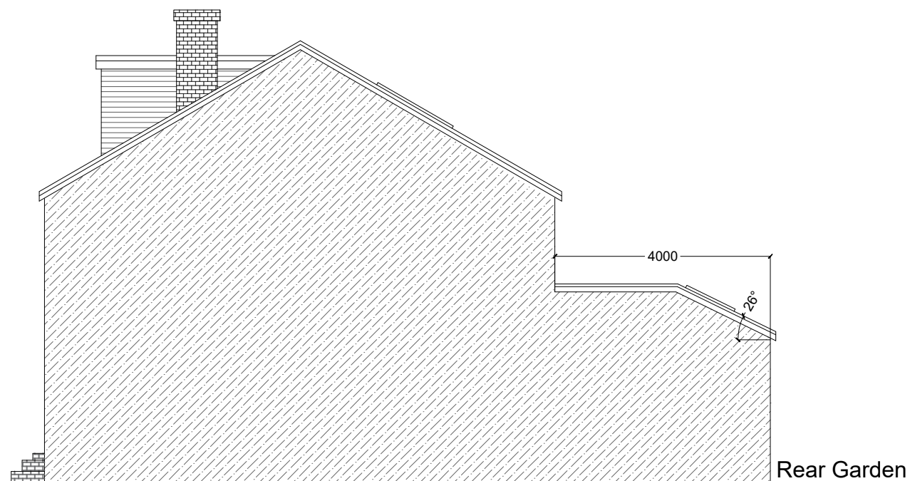
Proposed East Elevation 1:100 @A3
