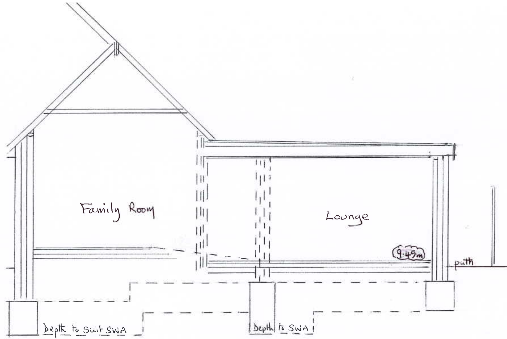
Section Y-Y
