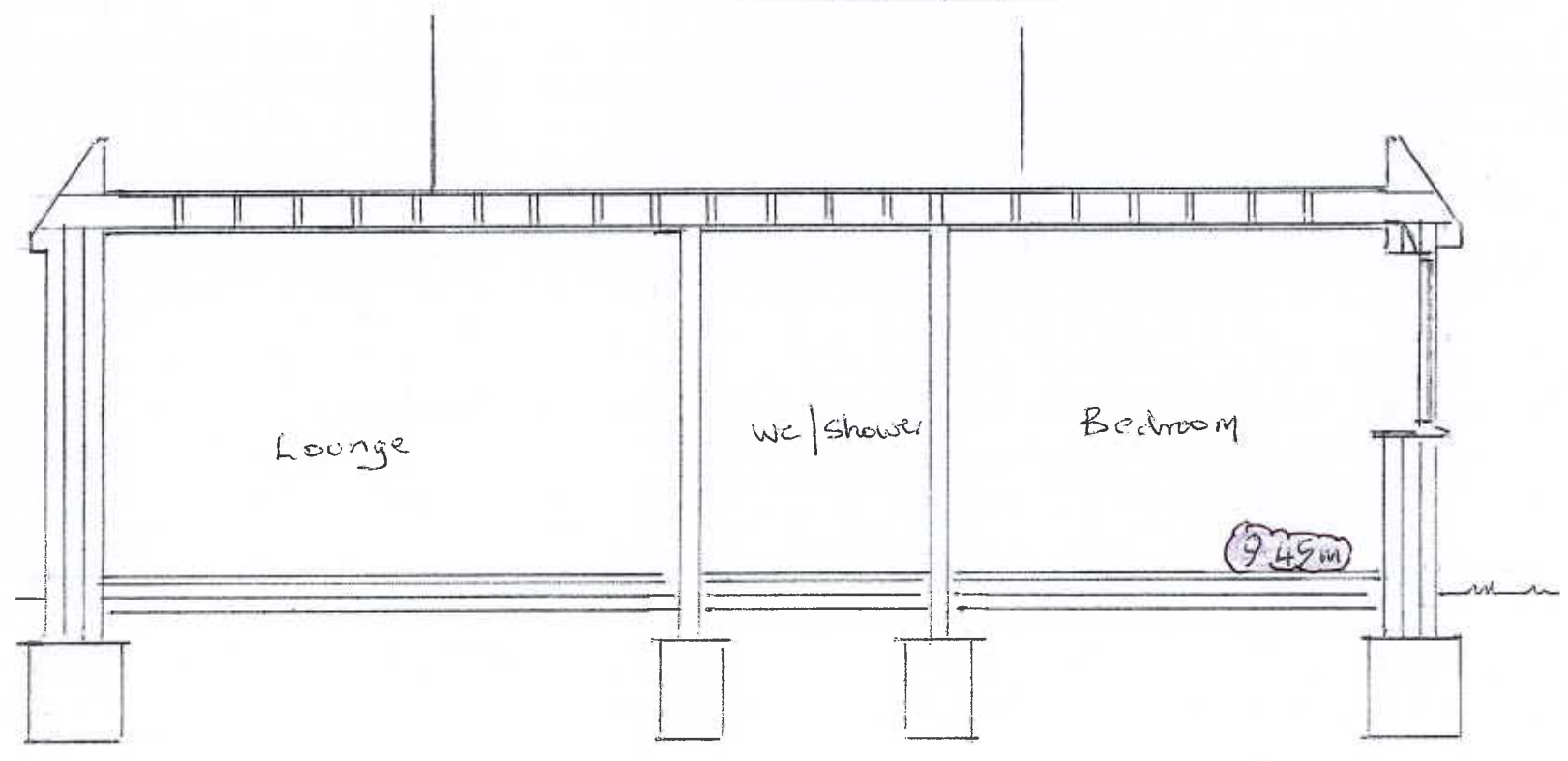
Section X-X 1:50
