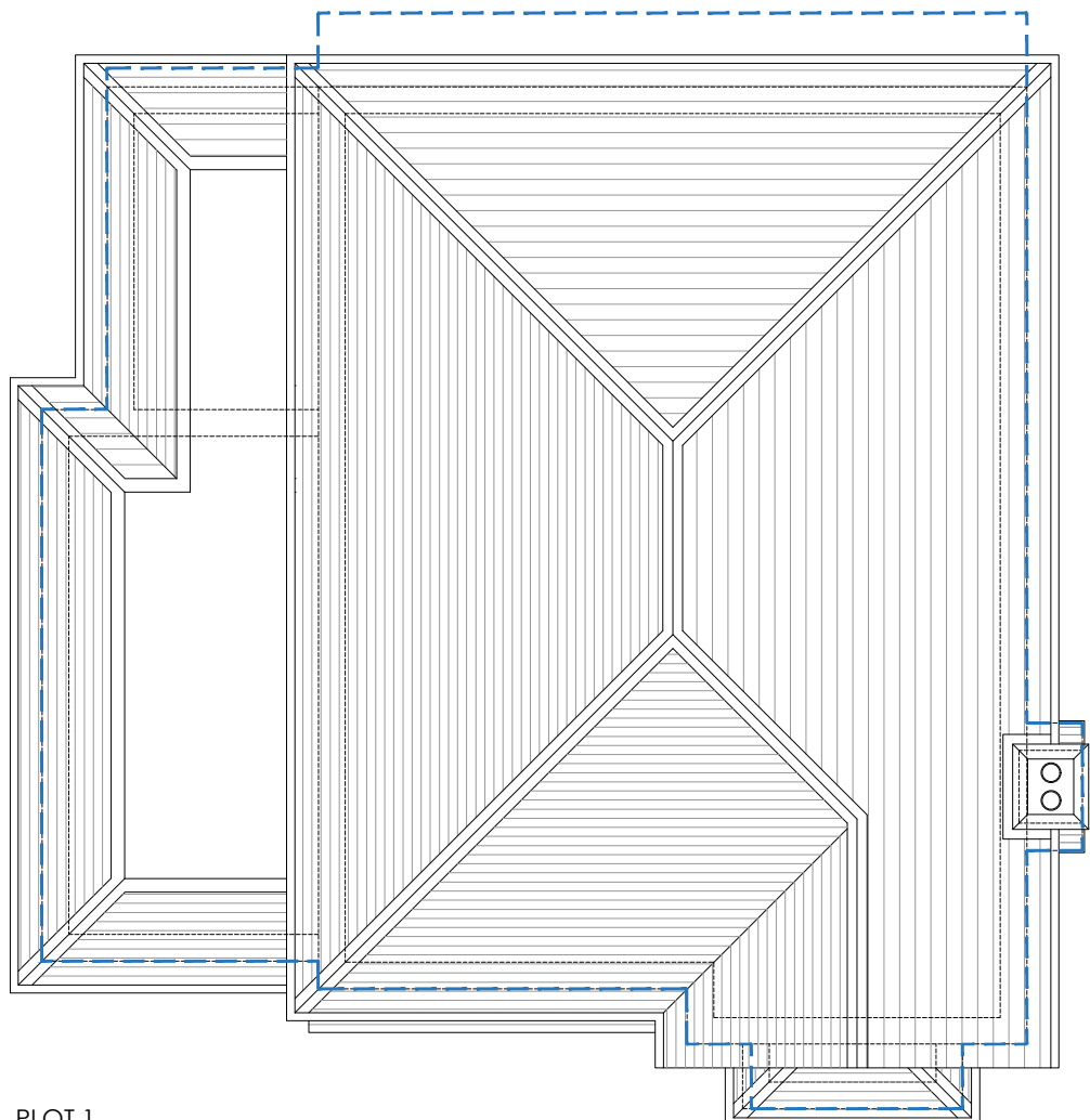
PLOT 1 As Proposed Roof Plan 1:100
