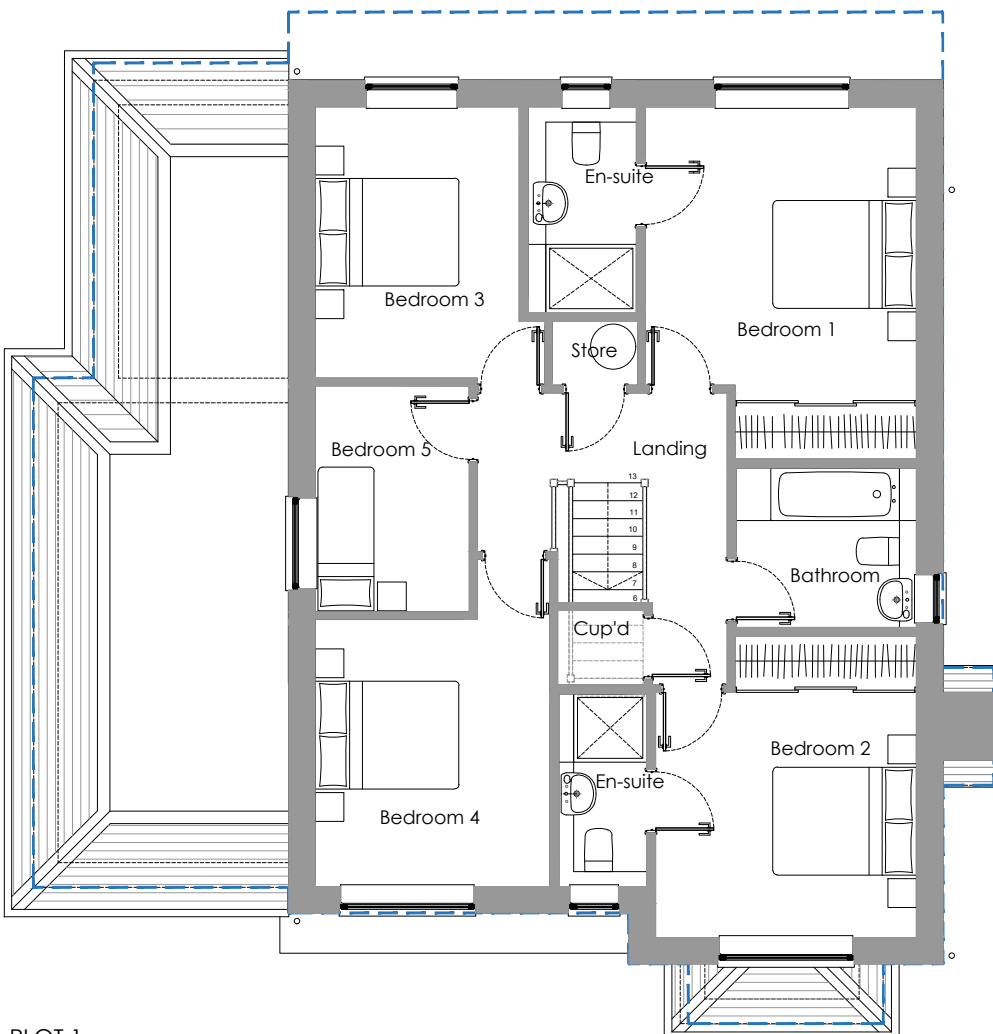
PLOT 1 As Proposed First Floor Plan 1:100
