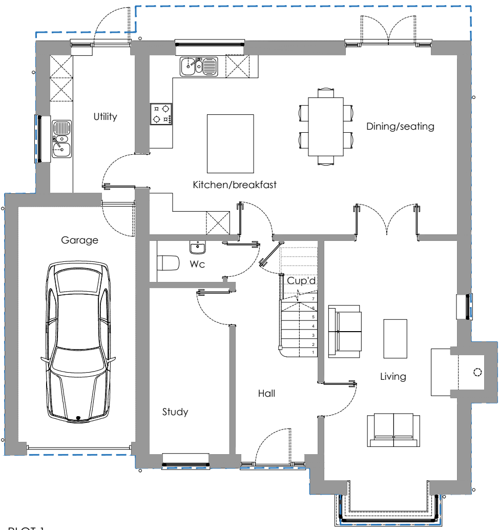
PLOT 1 As Proposed Ground Floor Plan 1:100
