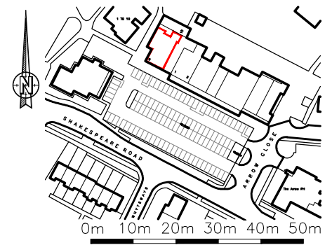
LOCATION PLAN @1:1250
