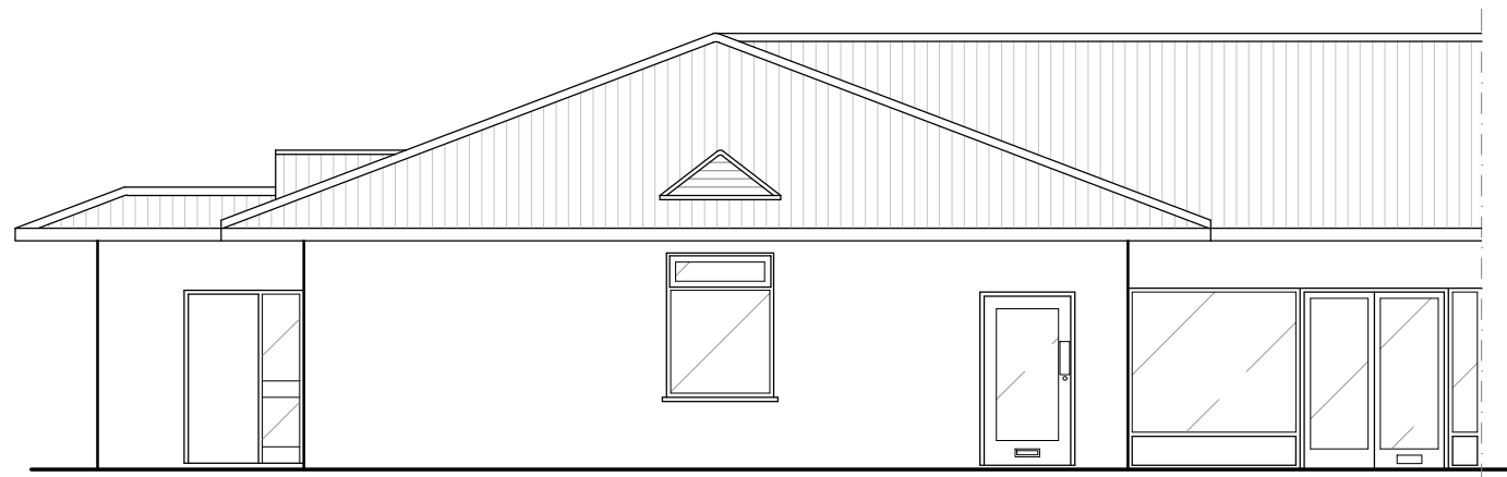
Existing Shop Front Elevation - 1:100
