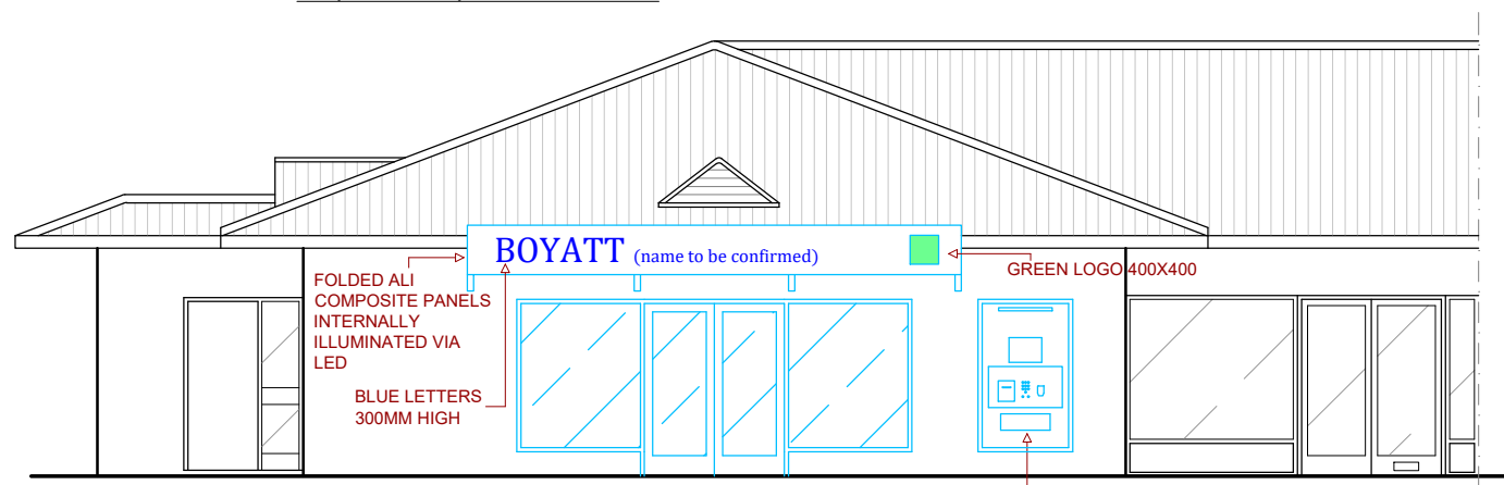
Proposed Shop Front Elevation - 1:100
