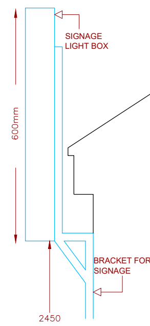
Proposed Signage Section - 1:10
