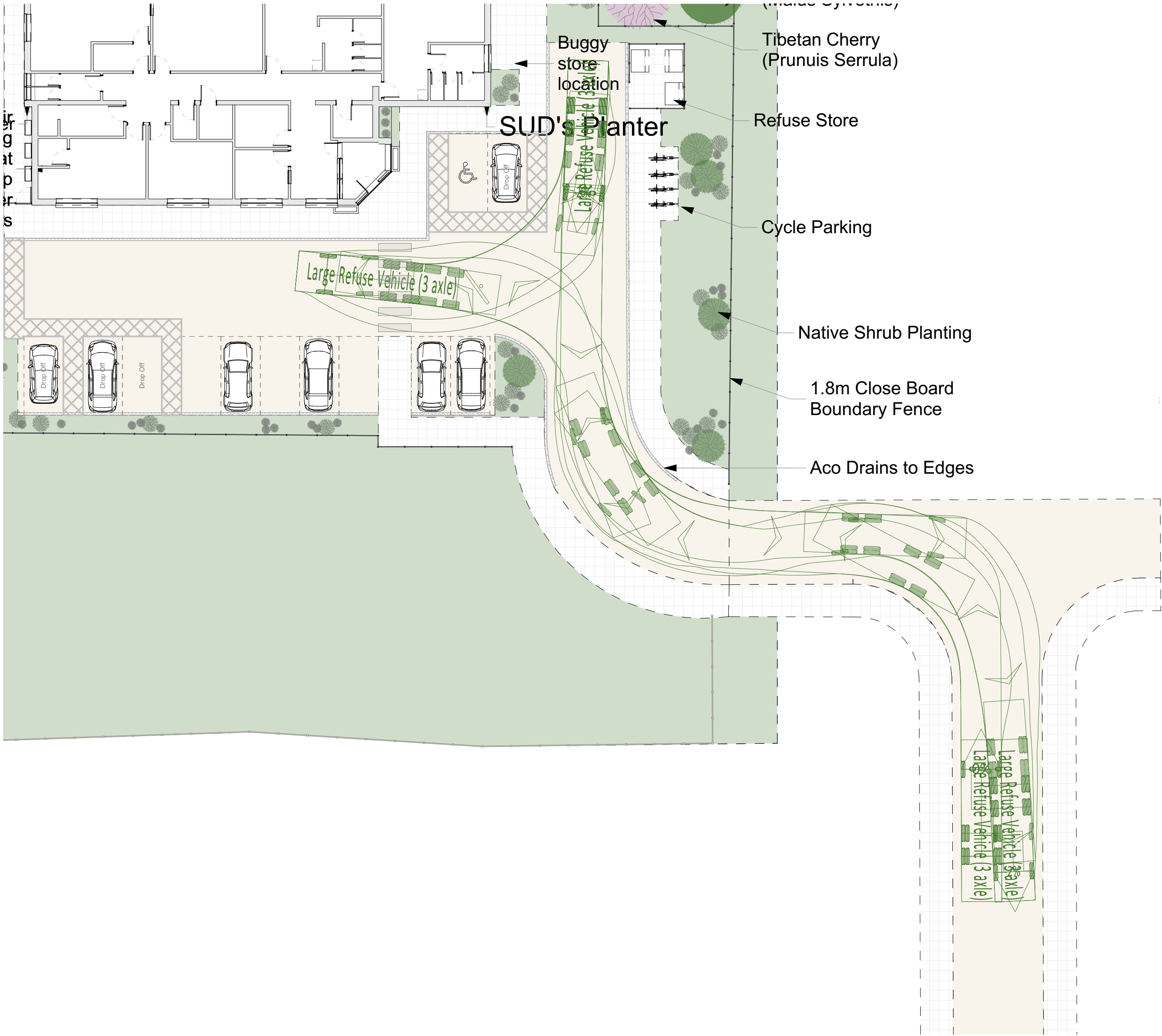
Proposed site plan with garbage truck 1:200
