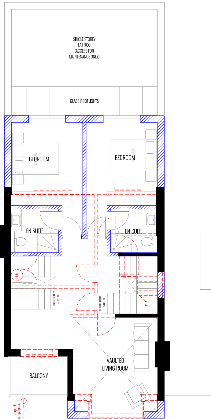
FIRST FLOOR | PROPOSED
