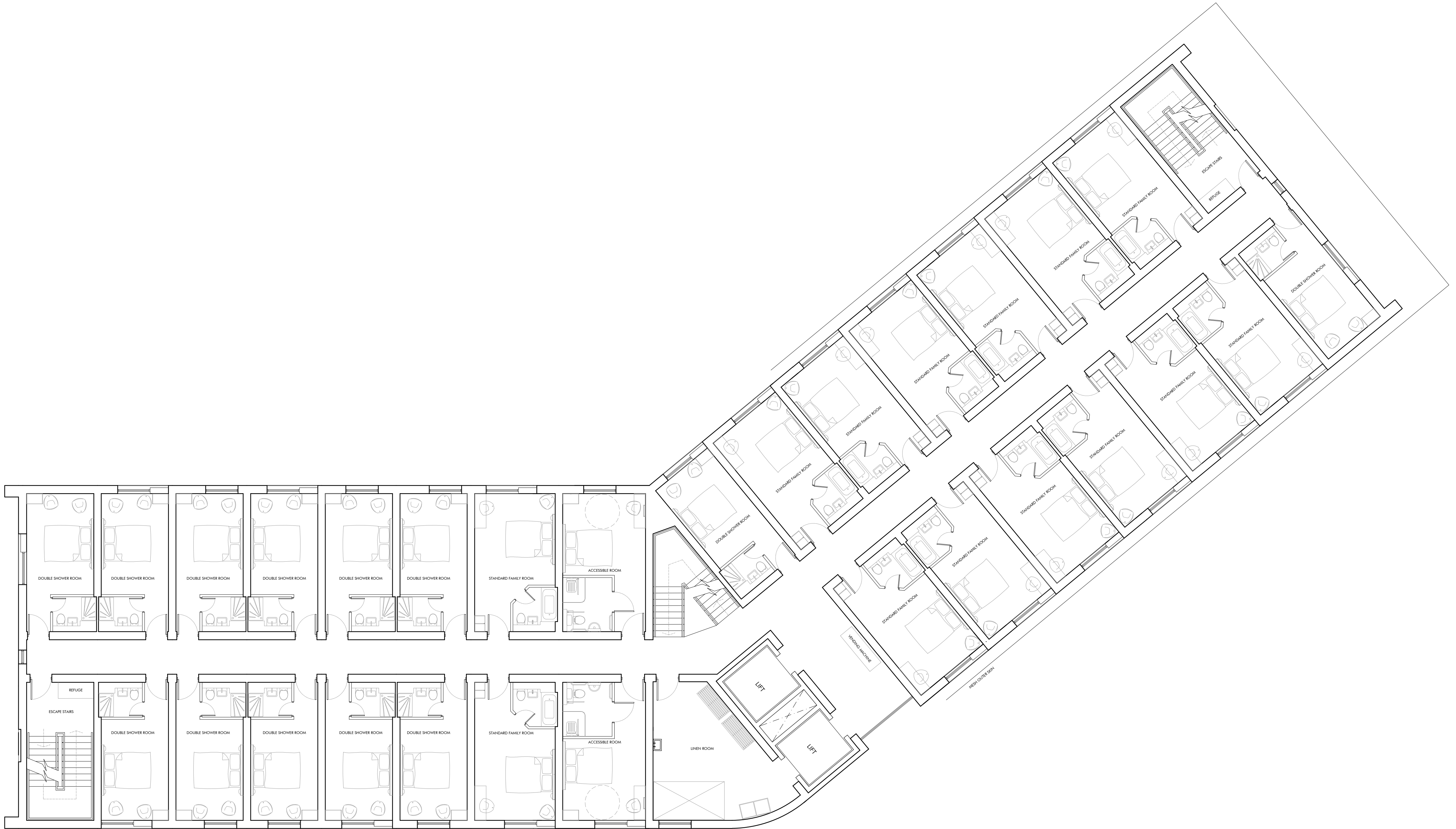
TYPICAL UPPER FLOOR PLAN
