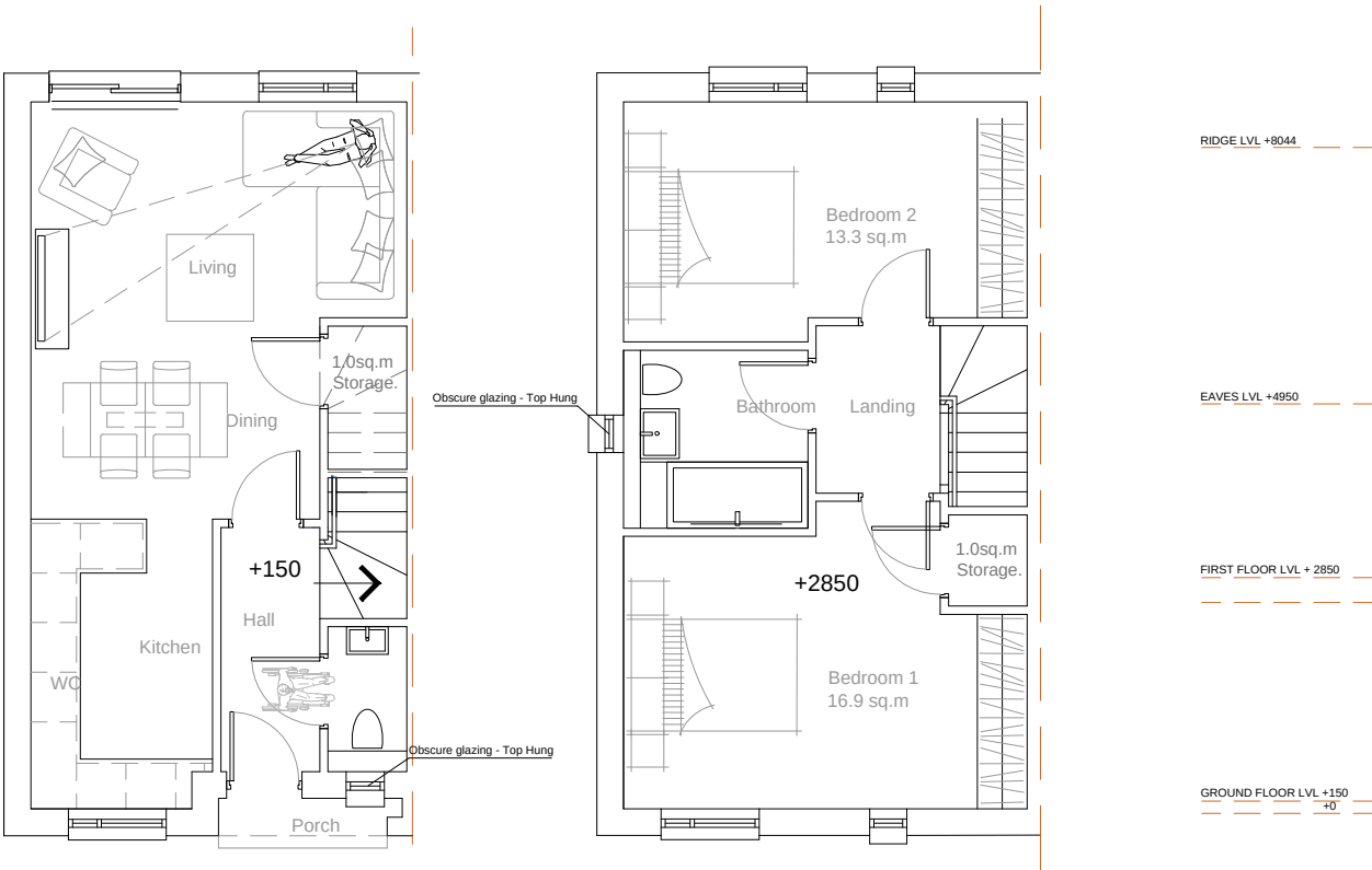
GROUND FLOOR 37.5sq.m. TOTAL 79sq.m. (850sq.ft)
