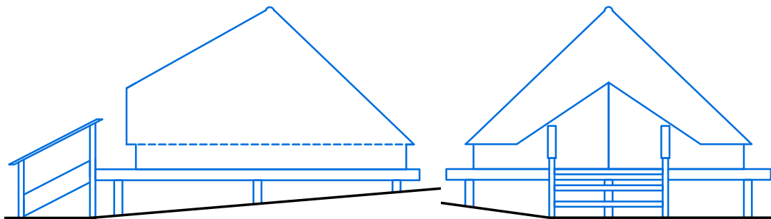
FRONT AND SIDE ELEVATION OF BELL TENT AND DECK
