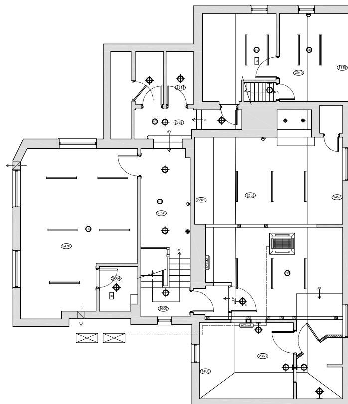
Proposed First Floor Reflected Ceiling Plan
