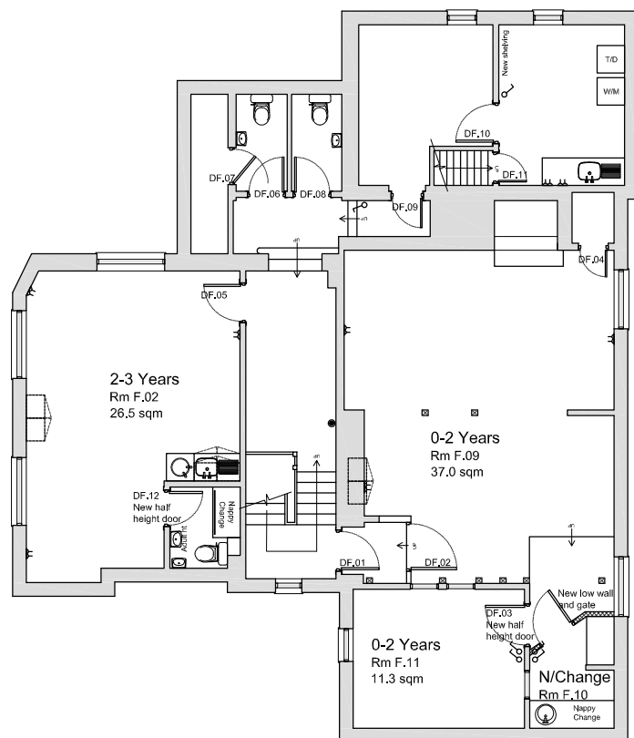
Proposed First Floor GA Plan
