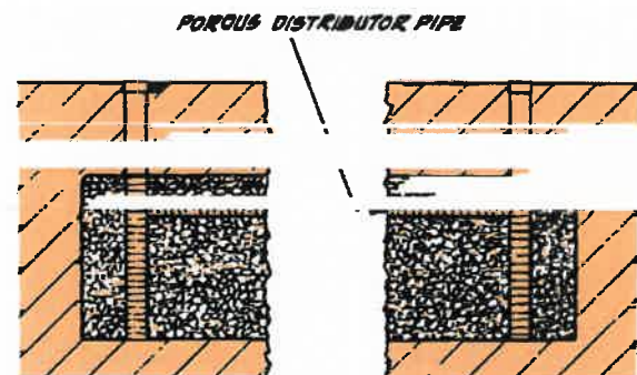
Figure 4 Trench type soakaway with horizontal distributor pipe
