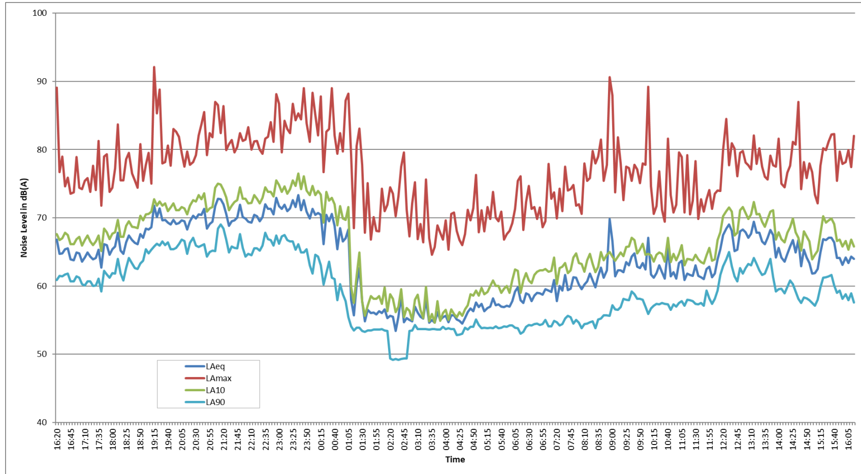
Figure 4.3: Noise Measurements – Measurement Location 2 (Side Façade)
