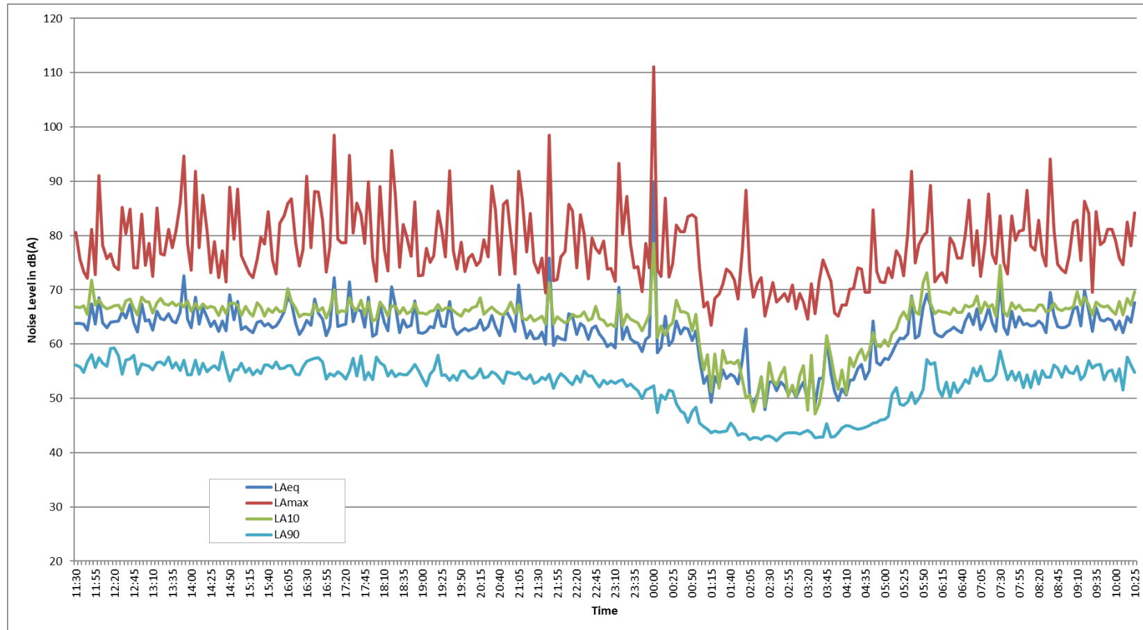
Figure 4.2: Noise Measurements – Measurement Location 1 (Front Façade)
