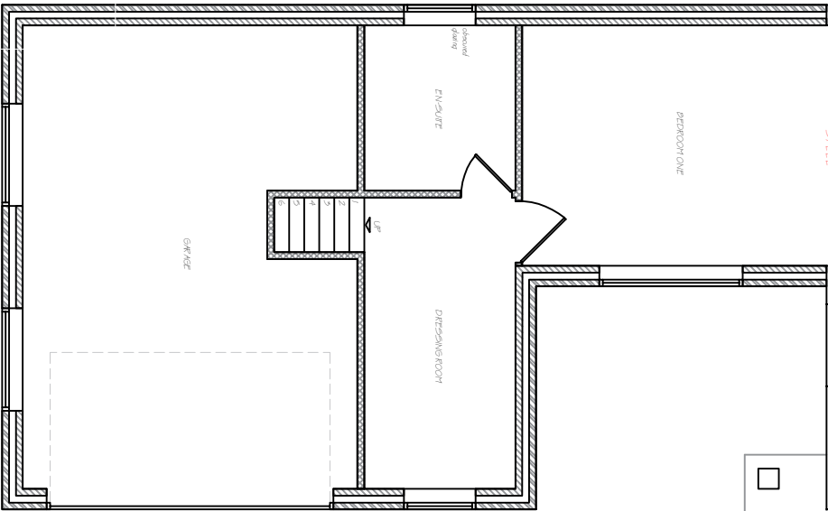
Proposed Ground Floor Plan 1 : 100 @ A3
